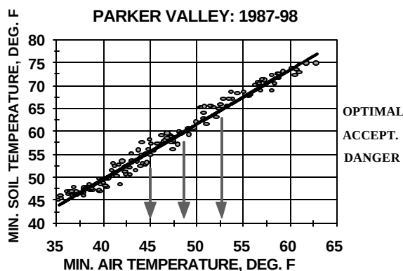
Fig. 1. Minimum soil vs. minimum air temperature for Parker Valley. Arrows indicate minimum temperatures associated with critical temperature thresholds for germination.
